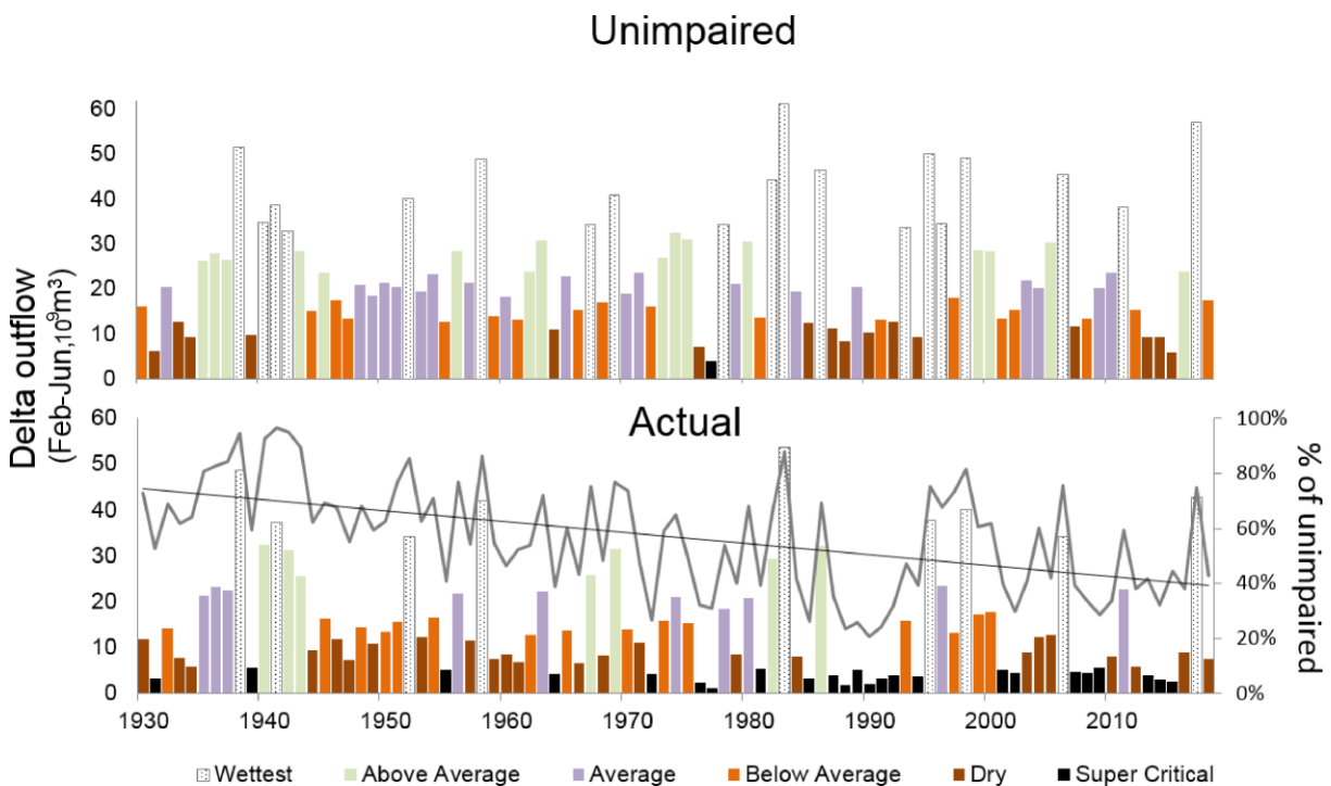
Figure 10: Trends in actual Delta outflow (below) relative to Central Valley unimpaired runoff (above). Coloring of bars represent water year types based on quintiles of unimpaired flow from 1922-2016. In terms of actual Delta outflow, the frequency of “wet” and “above normal” years is markedly reduced compared to unimpaired hydrology. The percentage of unimpaired flow reaching San Francisco Bay (line in lower panel; right y-axis) declined significantly during this
